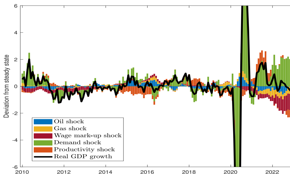
Figure E.1: Historical shock decomposition of real GDP growth in the euro area Note: Horizontal axis: months. Vertical axis: percentage-point deviations from the steady state.
